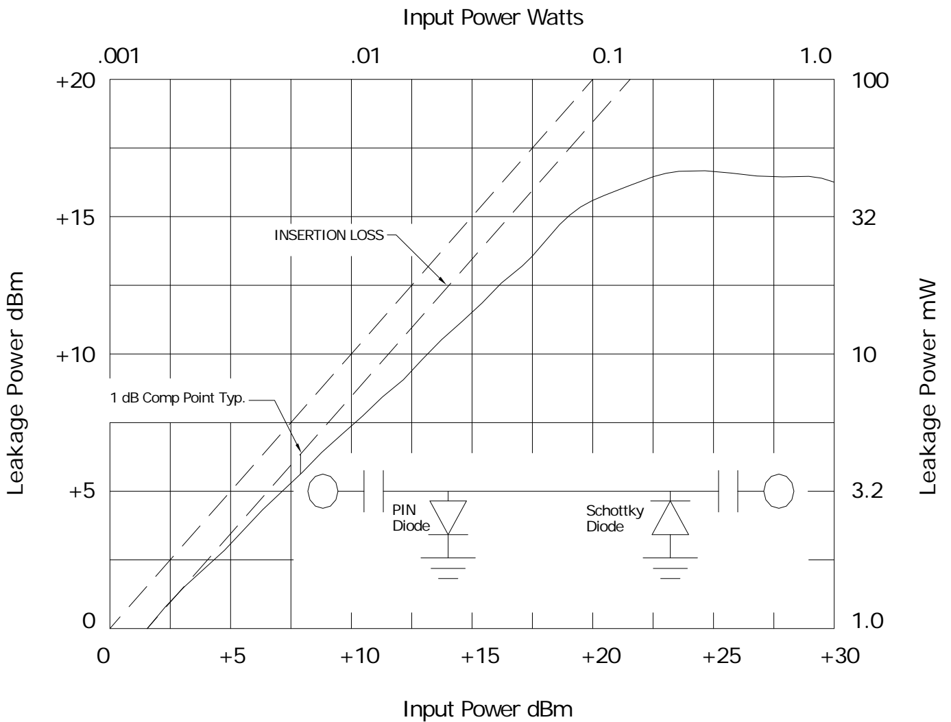
Typical ESL Curve
